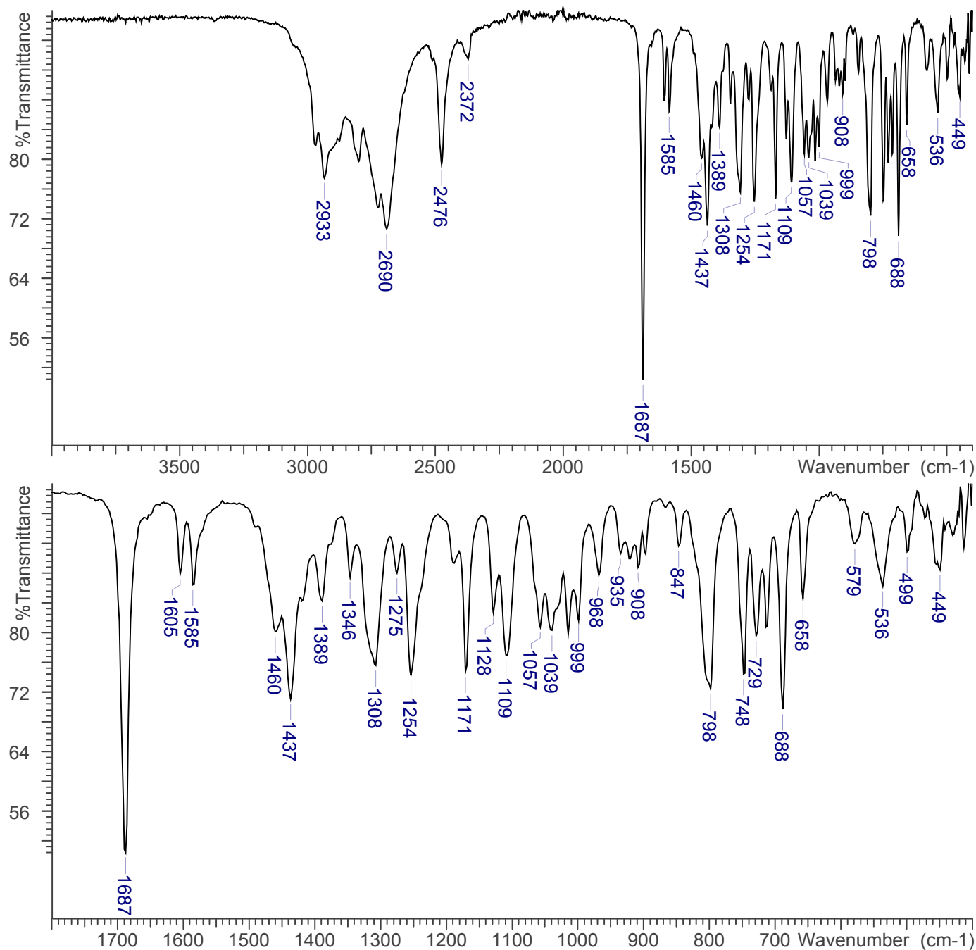
FTIR ATR (Diamond, 3 bounce): 3-ethylethcathinone HCl; lot 0435129-10
