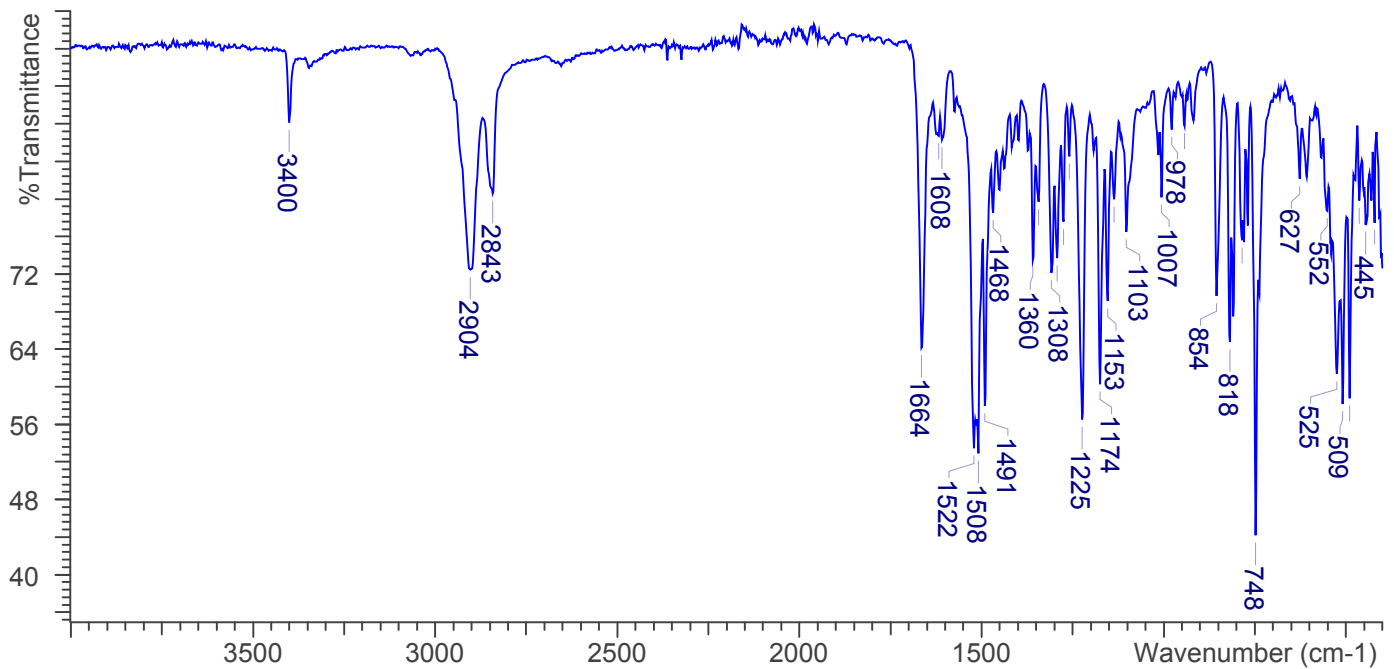
FTIR ATR (Diamond, 1 Bounce) FUB-AKB-48 Lot RM-131029-01
